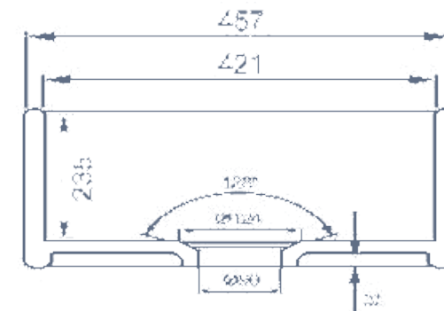
CROSS SECTION
