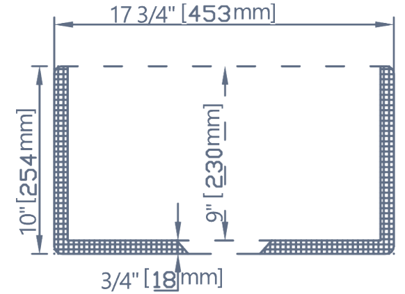
CROSS SECTION
